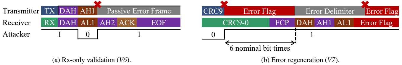
Figure 13: Error signalling enabled vulnerabilities.
