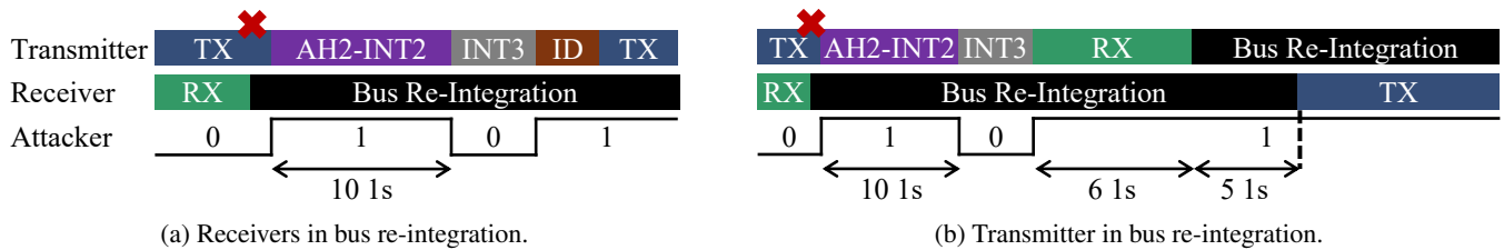
Figure 6: Tx/Rx state mismatch by injecting 0 in INT3 (V2.3).
