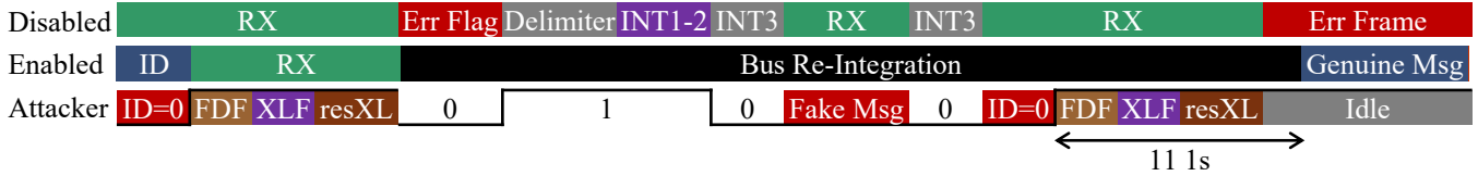
Figure 10: V4 exploit: inconsistent frames targeting XL enabled nodes with different protocol exception configurations.
