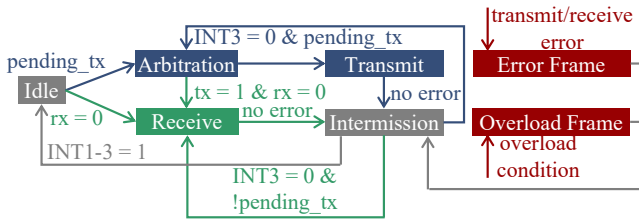
Figure 3: Simplified error signalling enabled state diagram.
